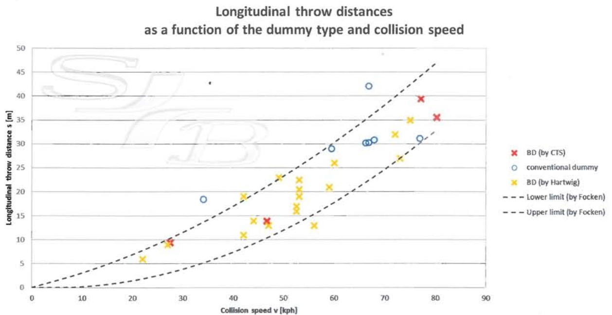
Figure 11: Graph with throw distances of the different dummy types as a function of the collision velocity – trend line according to Focken 6
