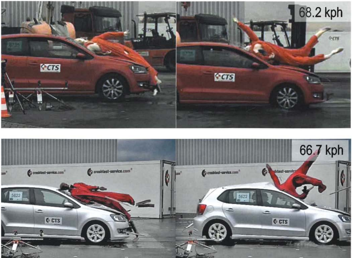
Figure 10: Deformation of the roof edge after an impact with the biofidelic dummy (top) and a conventional dummy (bottom) at approx. 70 kph
